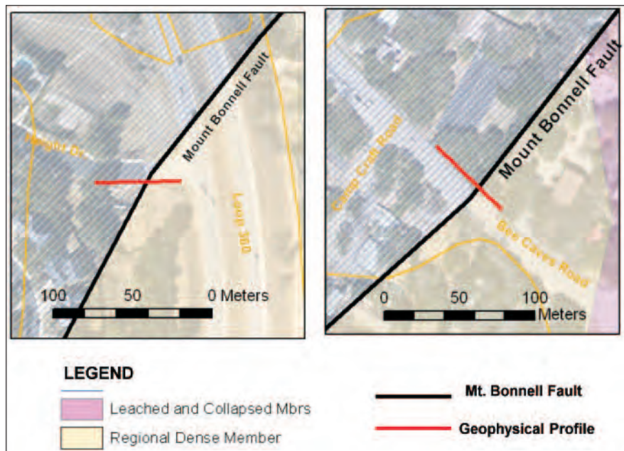
Figure 2: Surface geology of geophysical survey sites. Geologic interpretation modified from Hauwert, 2009 and Rodda et al. (1970) by Nico Hauwert.
